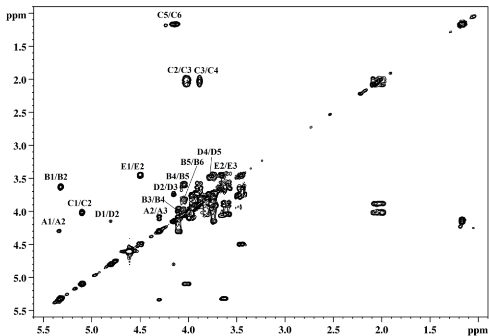
Fig. 2S. The COSY spectrum of the OPS isolated from Pectobacterium aquaticum IFB5637. The letters refer to the monosaccharides residues as defined in Table 1 , and the Arabic numerals refer to the protons in the respective residues.
